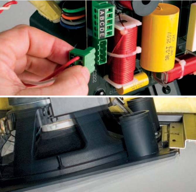
EZ-RAIL™ PROVIDES A "HELPING HAND" DURING INSTALLATION
